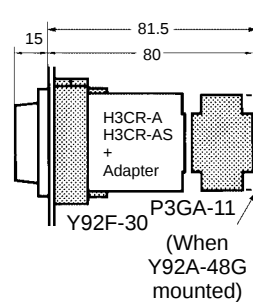
Dimensions with Back Connecting Socket P3G-08/P3GA-11
