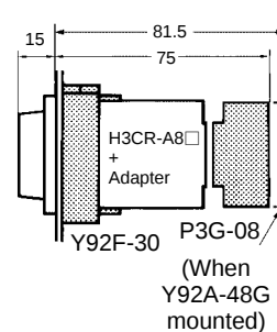
Dimensions with Back Connecting Socket P3G-08/P3GA-11
