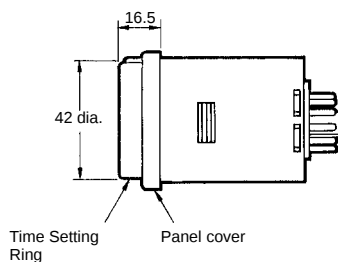
Dimensions with Back Connecting Socket P3G-08/P3GA-11
