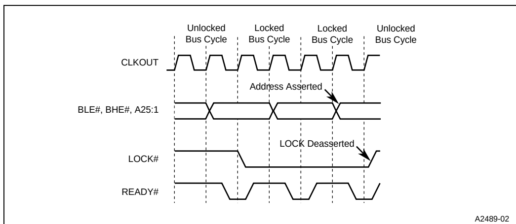
Figure 29. LOCK# Signal During Address Pipelining
