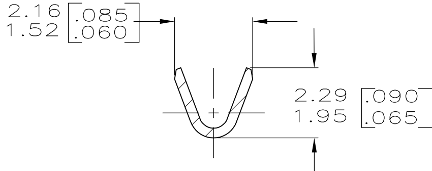
SECTION B-B SCALE 10:1
