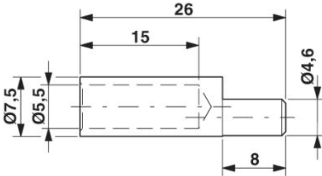
Dimensional drawing
