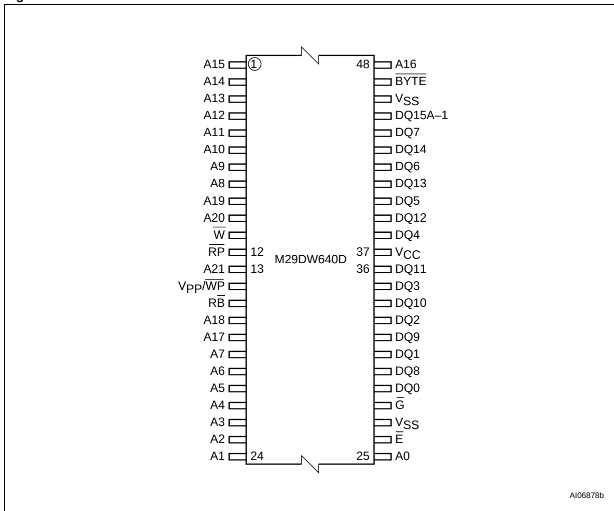
Figure 3. TSOP Connections
