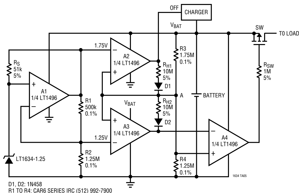
Single Cell Li-Ion Battery Supervisory Circuit ( I_0 = 20\mu\text{A} )
