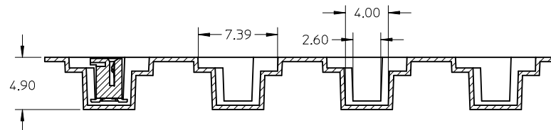
SECTION Z-Z
