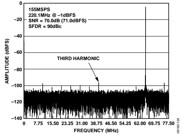
Figure 28. AD9644-155 Single-Tone FFT with f_{IN} = 220.1 MHz
