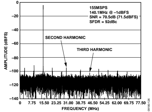
Figure 26. AD9644-155 Single-Tone FFT with f_{IN} = 140.1 MHz
