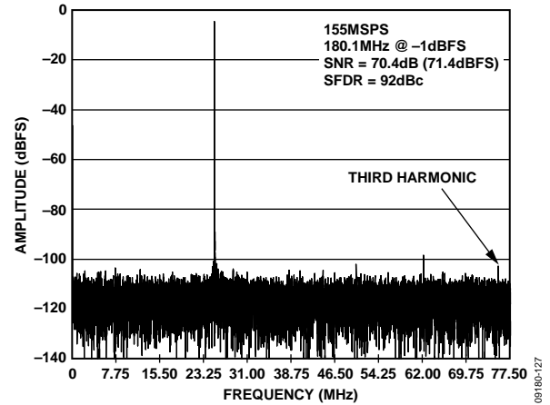
Figure 27. AD9644-155 Single-Tone FFT with f_{IN} = 180.1 MHz
