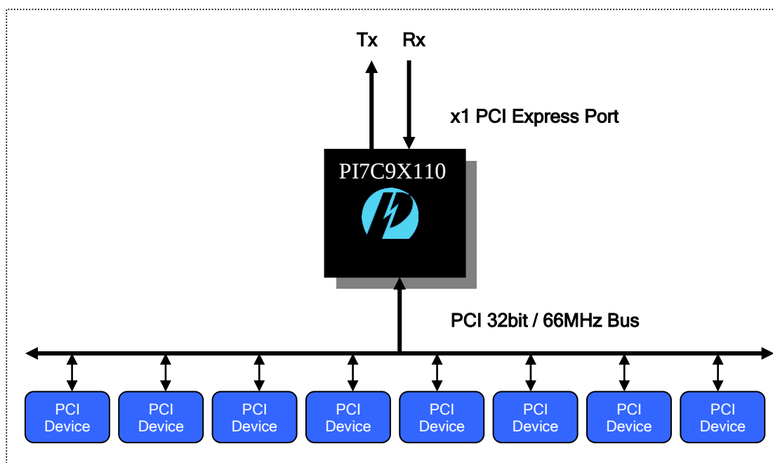
Figure 1-1 PI7C9X110 Topology
