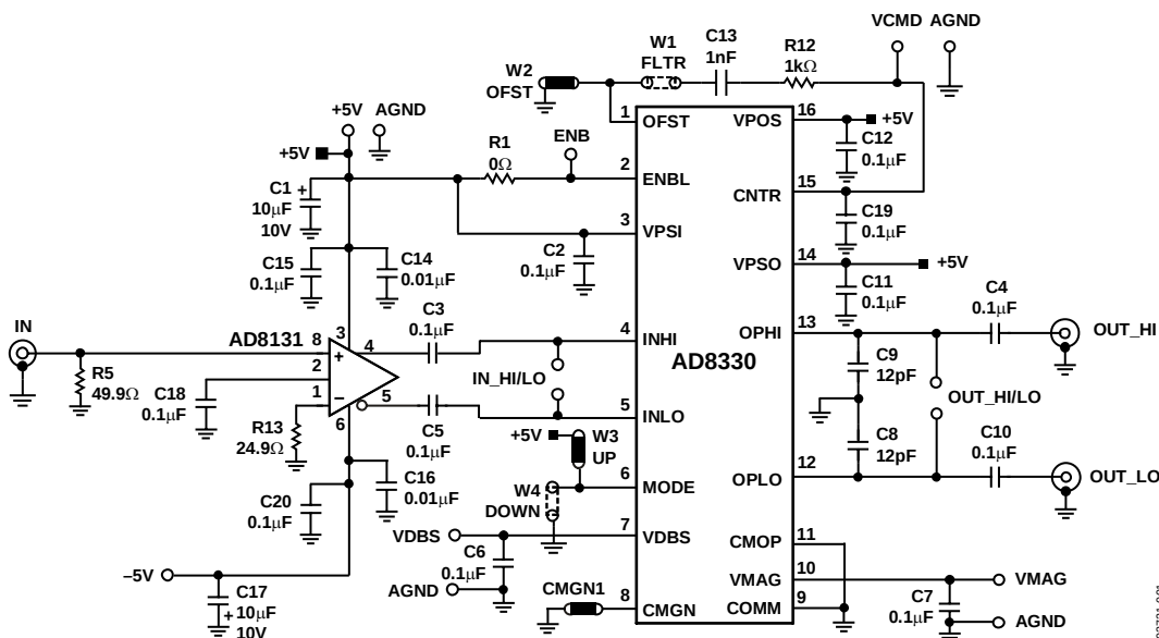
Figure 2. Schematic Diagram
