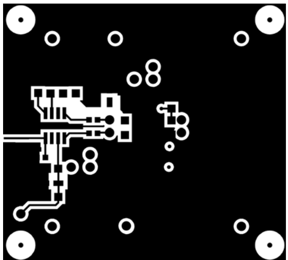
Figure 8. Wiring-Side Pattern
