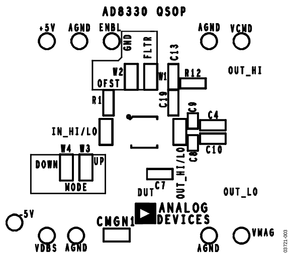
Figure 4. Component-Side Silkscreen
