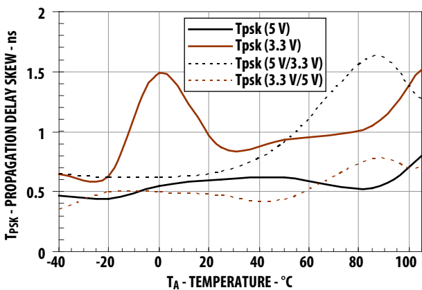
Figure 12: Typical Channel-Channel Delay Skew vs. Temperature
