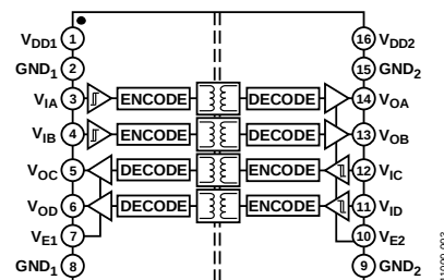
Figure 3. ADuM3402W Functional Block Diagram
