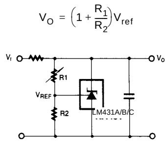
Figure 11. Shunt Regulator
