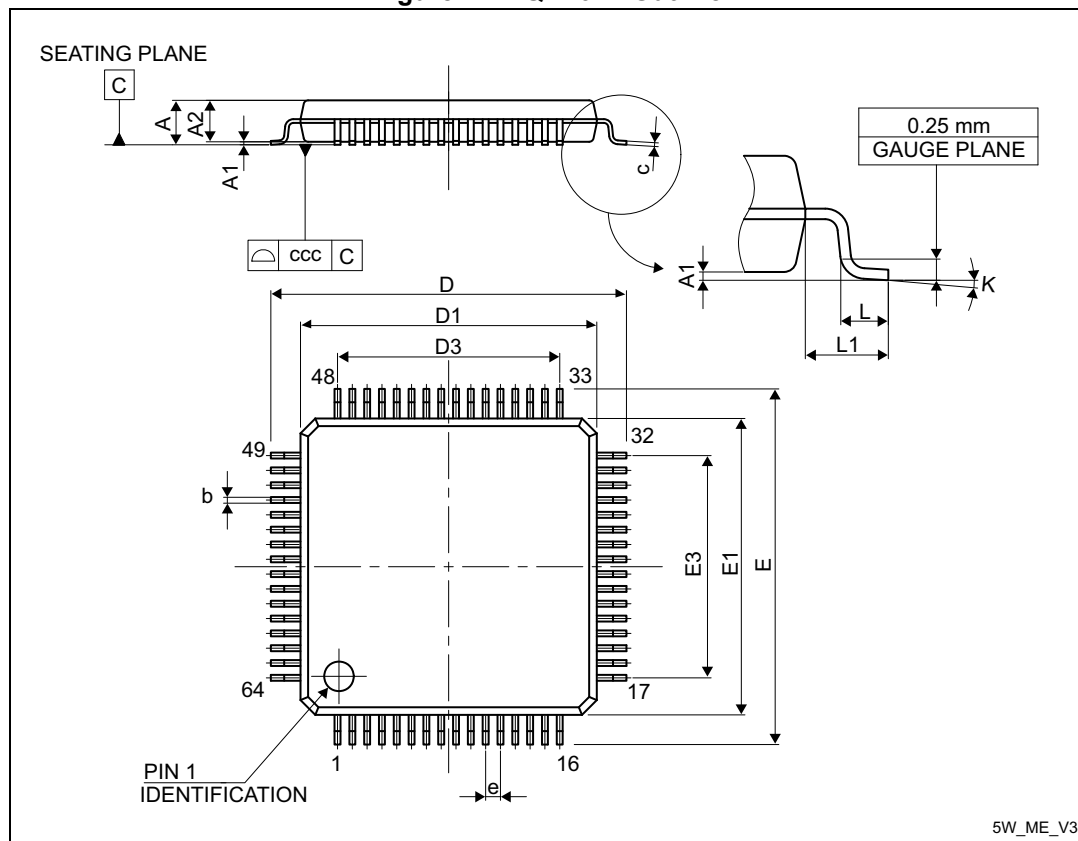
Figure 47. LQFP64 - Outline
