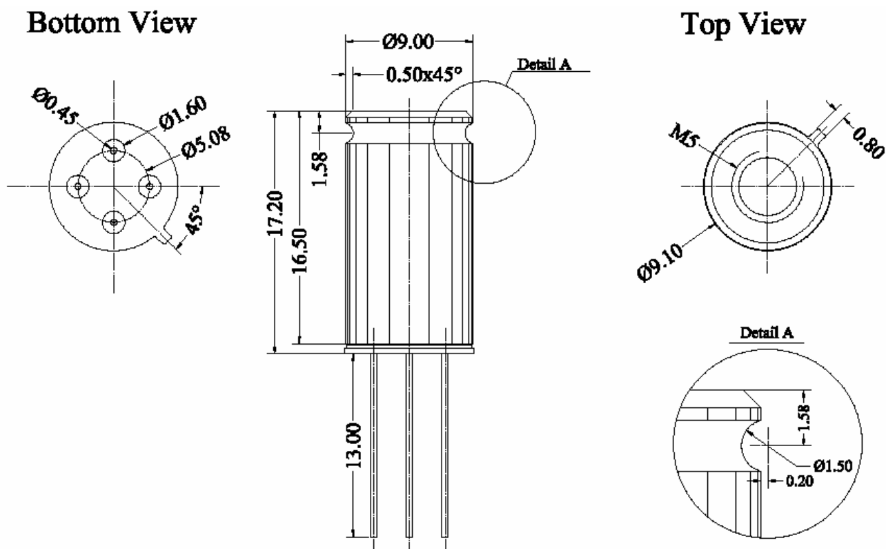
Figure 31: MLX90614XCF package
