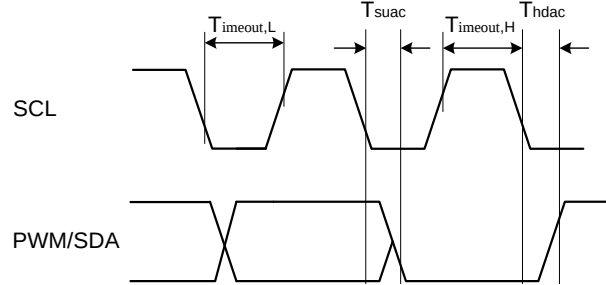
Figure 7: SMBus timing
