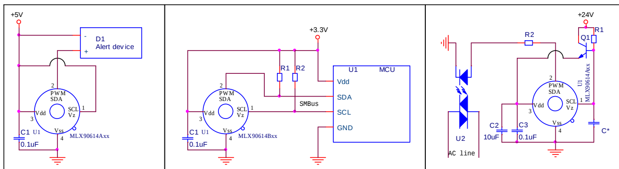
Figure 27: Thermal alert/thermostat applications of MLX90614
