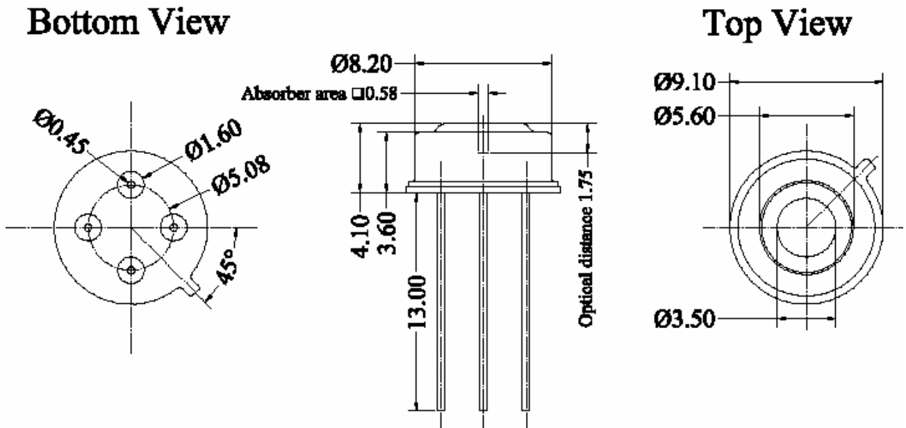
Figure 29: MLX90614XXA package
