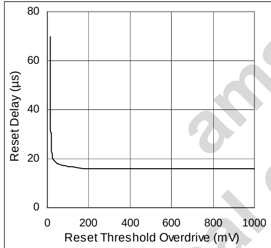
Figure 5. Reset Delay vs. Reset Threshold Overdrive; V_{IN2} = 3.0\text{V} , IN decreasing
