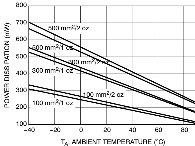
Figure 6. Power Dissipation vs. Ambient Temperature @ T_J = 150 °C
