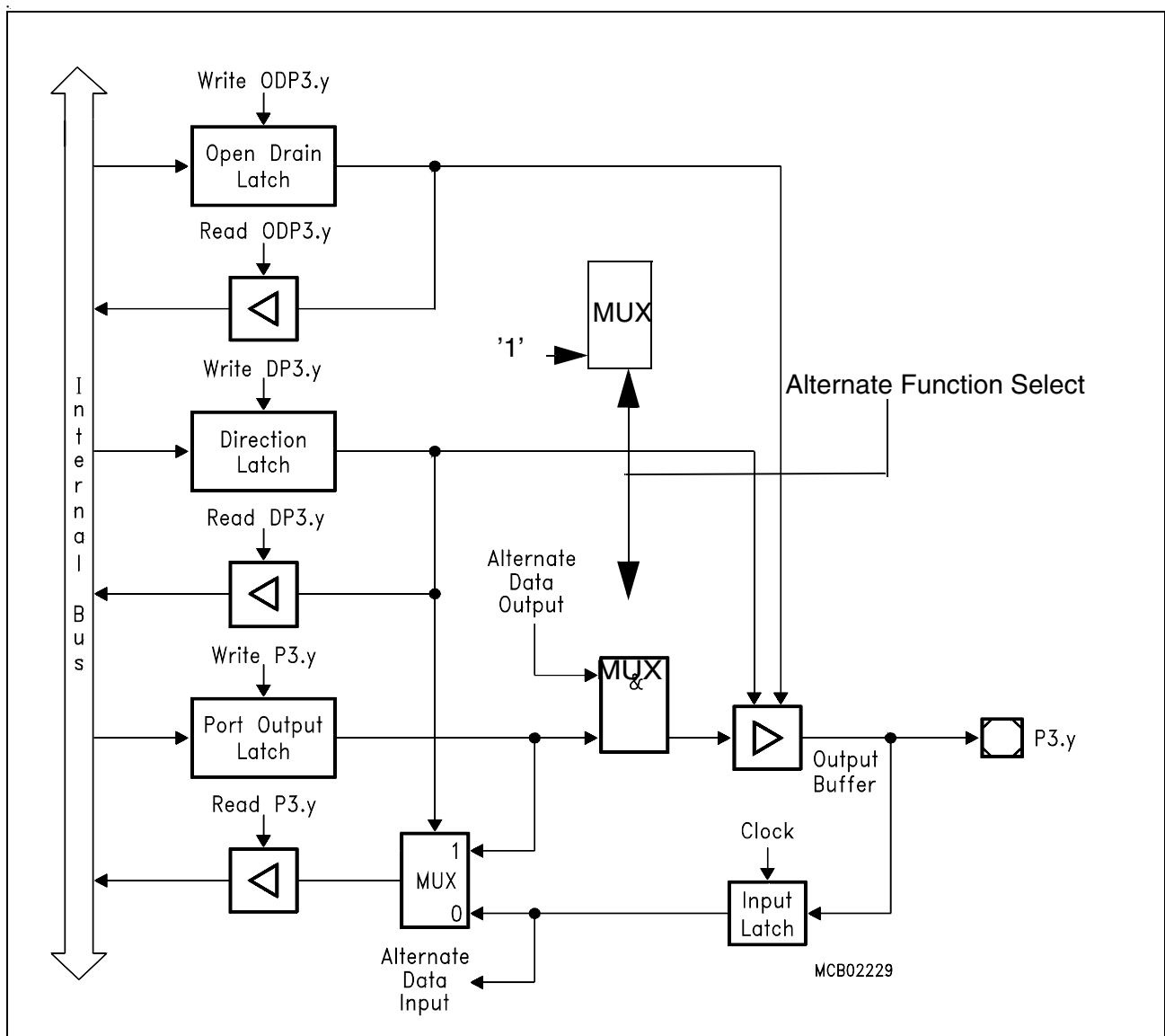
Figure 9-3 Port structure
