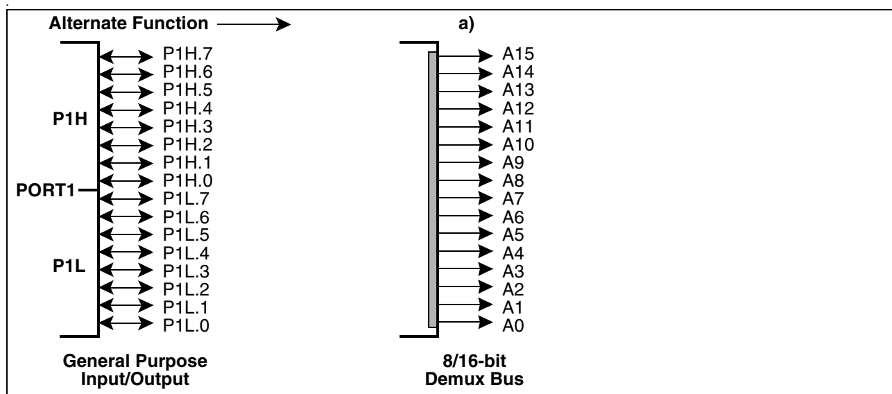
Figure 9-5 PORT1 I/O and Alternate Functions
