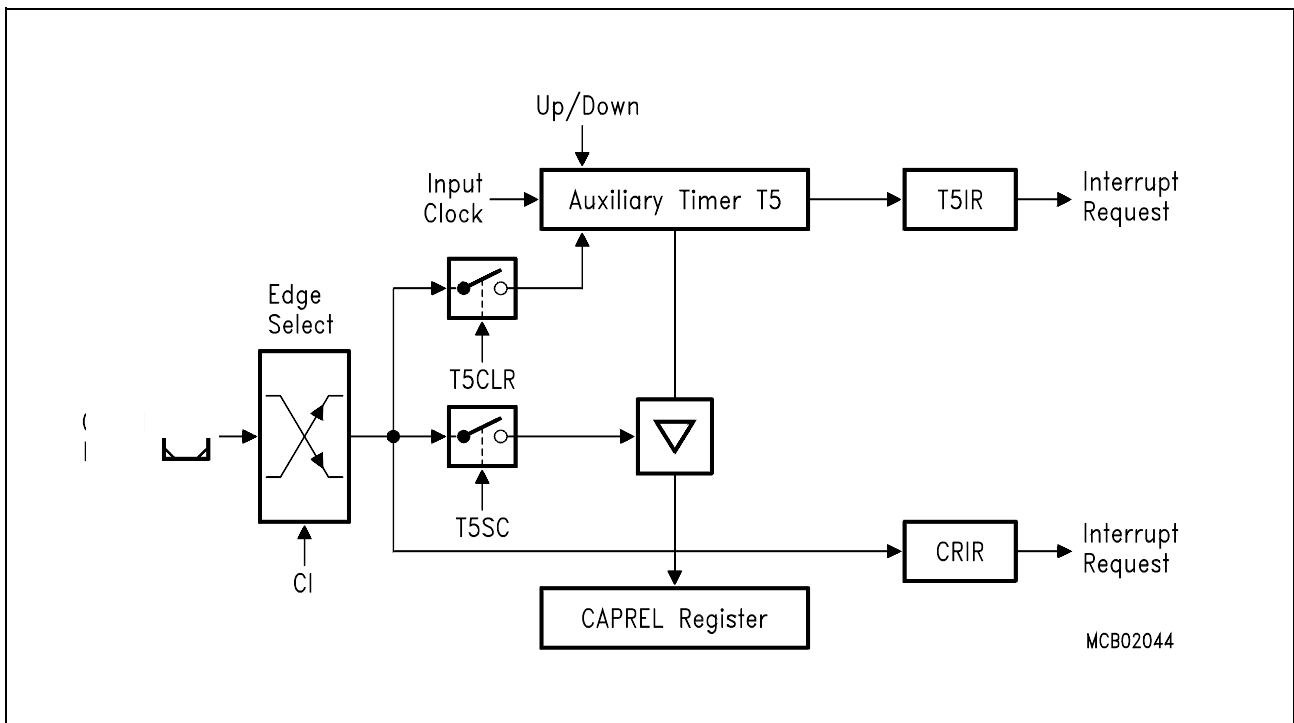
Figure 14-21 Timer Block 2 Register CAPREL in Capture Mode
