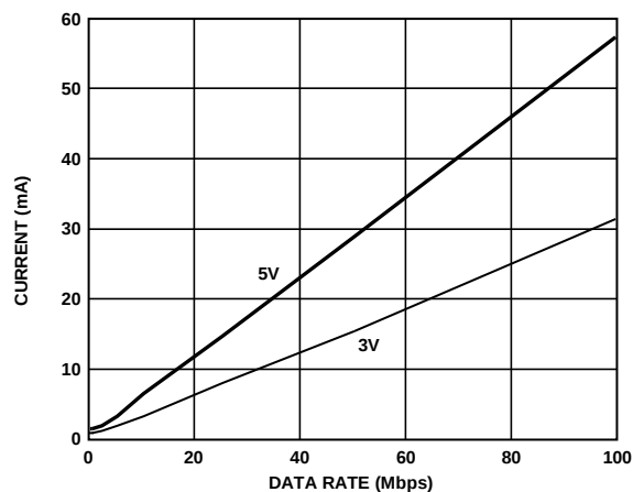
Figure 9. Typical ADuM1300 V_{DD1} Supply Current vs. Data Rate for 5 V and 3 V Operation
