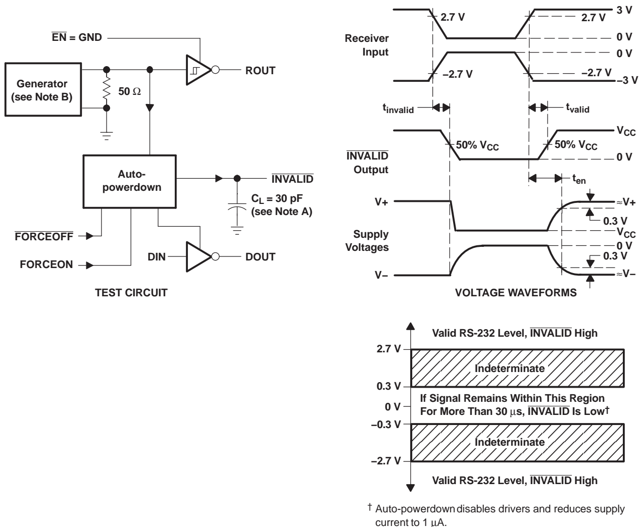
Figure 5. \text{INVALID} Propagation Delay Times and Driver Enabling Time
