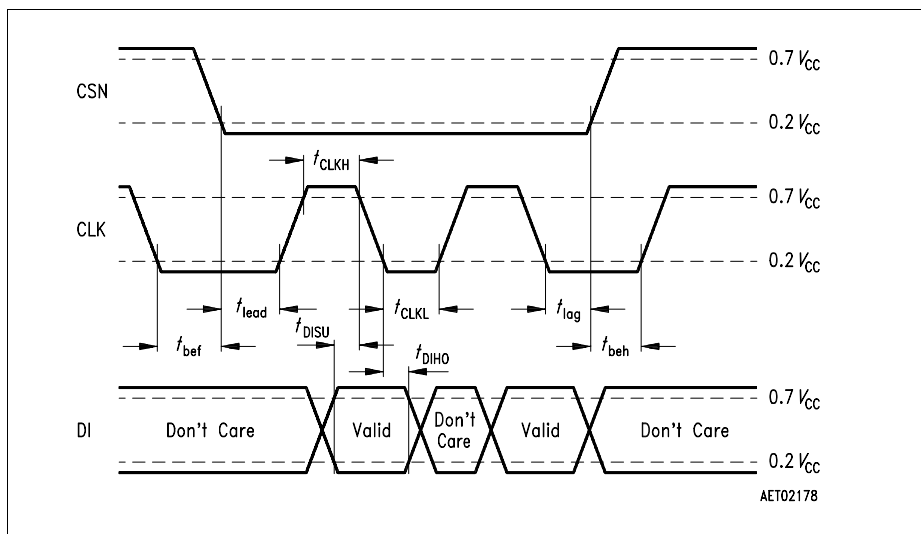
Figure 13 SPI-Input Timing
