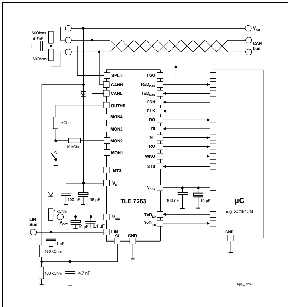
Figure 22 Application Circuit
