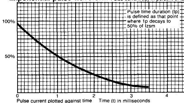
Exponential pulse waveform Pulse current ( I_p ) in percent of I_{zsm}
