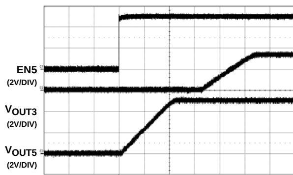
FIGURE 24. DELAYED START WAVEFORMS (EN3 = REF)
