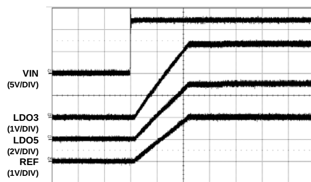
FIGURE 22. REF, LDO3, AND LDO5 POWER-UP
