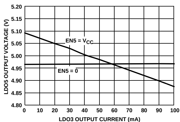
FIGURE 20. LDO5 REGULATION OUTPUT VOLTAGE vs OUTPUT CURRENT
