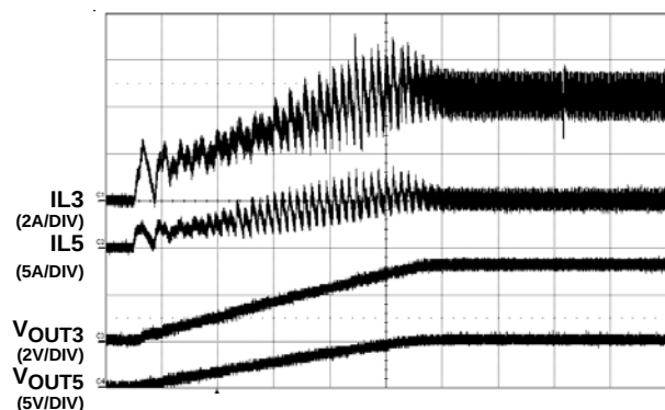
FIGURE 25. SOFT-START WAVEFORMS
