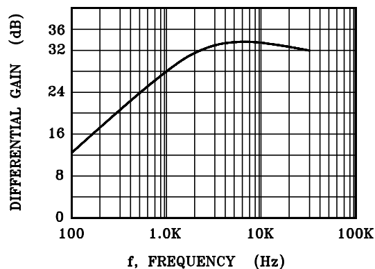
FIGURE23-FREQUENCY RESPONSE OF FIGURE22
