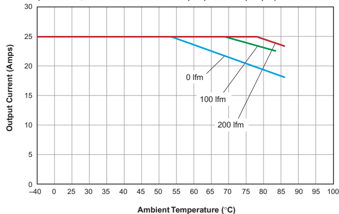
Output Current vs. Ambient Temperature ( V_{IN} = 48V , air flow direction from Input pin to Output pin)
