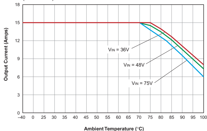
Output Current vs. Ambient Temperature (No air flow)
