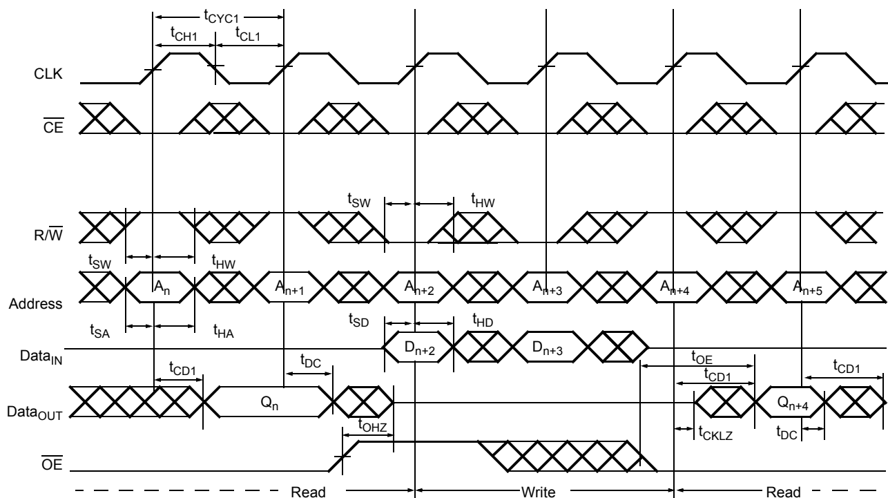
Figure 14. Flow-Through Read-to-Write-to-Read ( \overline{OE} Controlled) [42, 43, 46, 47, 48]
