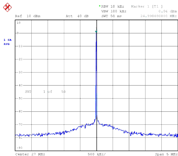
Figure 9-6. f out = 27MHz, VCO frequency < 125MHz, SSC (2% center)
