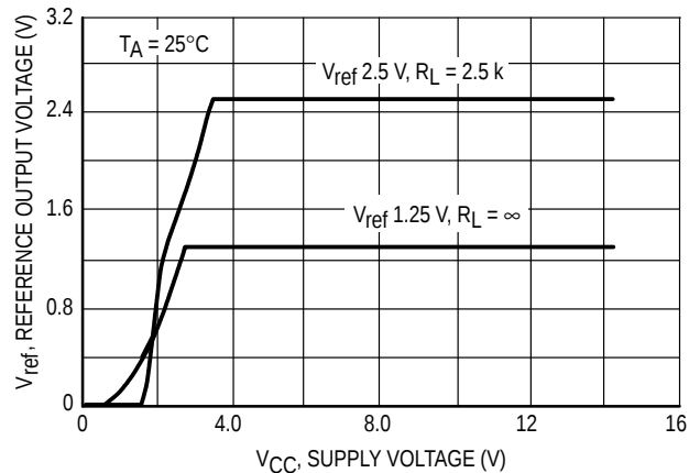
Figure 10. Reference Output Voltage versus Supply Voltage
