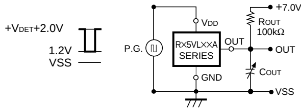
FIG. 7 Output Delay Time Test Circuit
