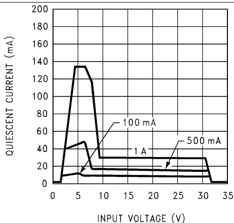
Figure 5. Quiescent Current
