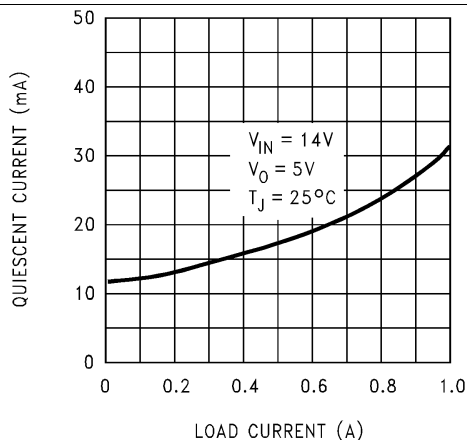
Figure 6. Quiescent Current
