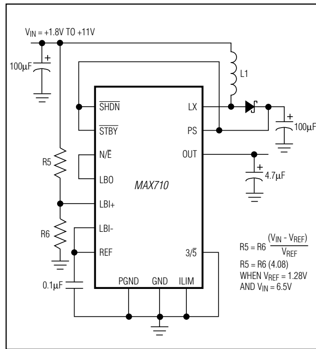
Figure 2b. High-Efficiency Operating Configuration for V_{BATT} < 6.5V
