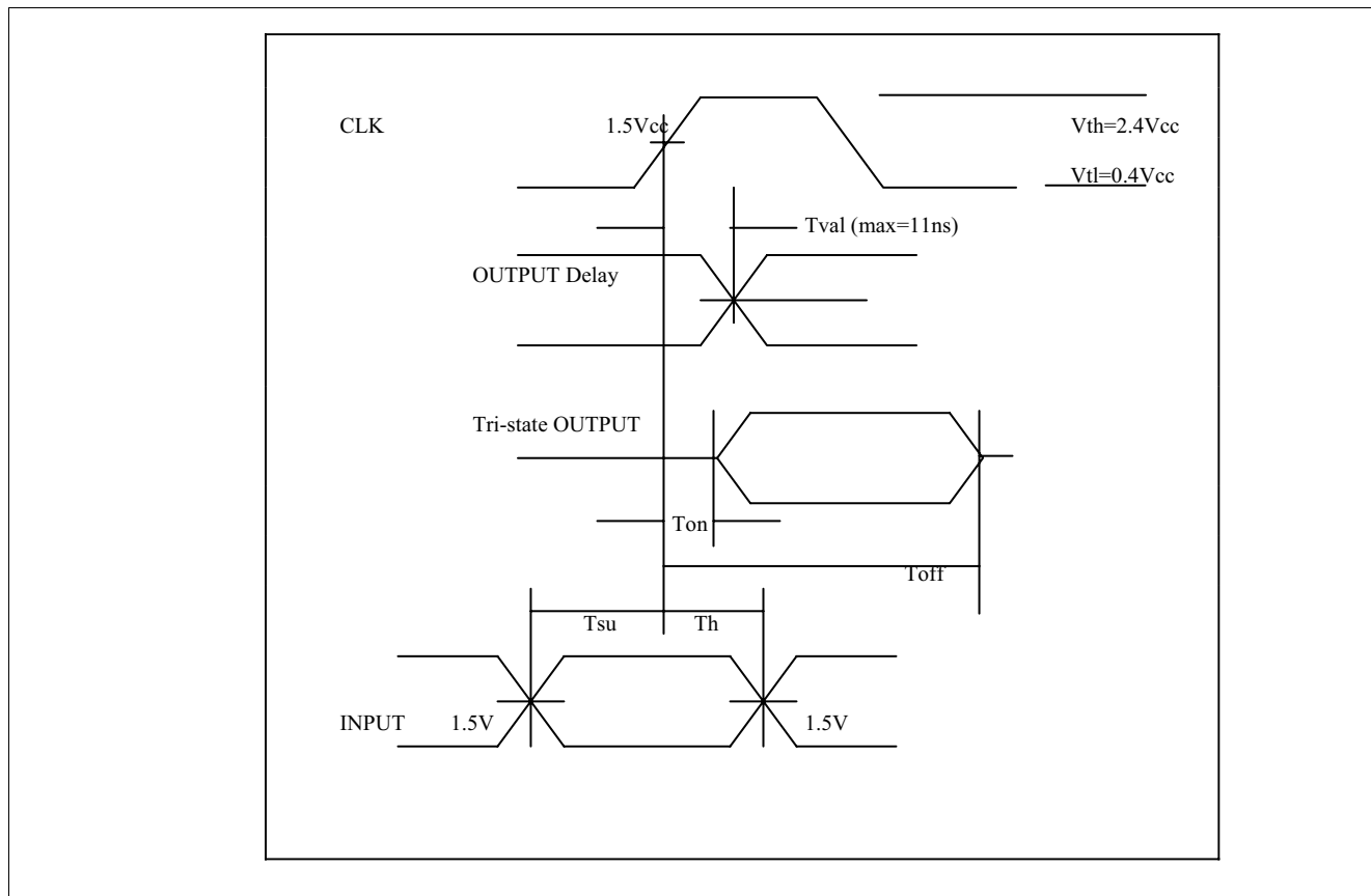
Figure 18 PCI Timings
