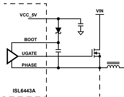
FIGURE 15. GATE DRIVER
