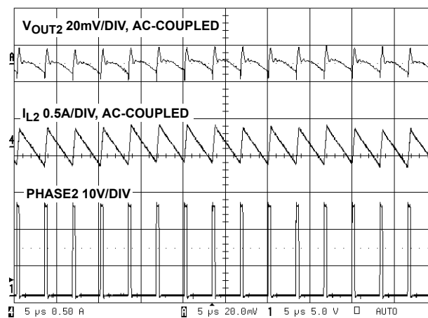
FIGURE 6. PWM2 WAVEFORMS
