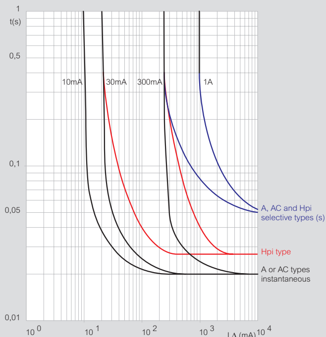
Average residual current performance curves
