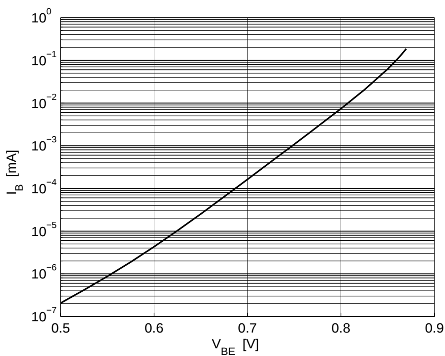
Figure 5-5 Base Current vs. Base Emitter Forward Voltage I_B = f(V_{BE}) , V_{CE} = 1.8 V
