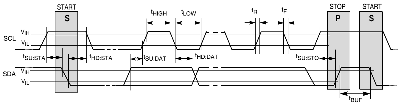
FIGURE 6. BUS TIMING
