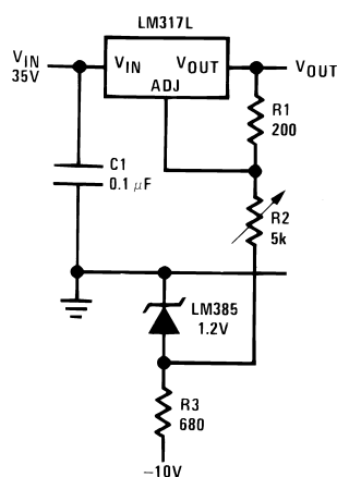
Figure 27. 0V–30V Regulator
