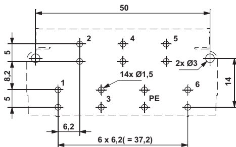
Drilling diagram
