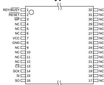
TSOP Top View Type 1
