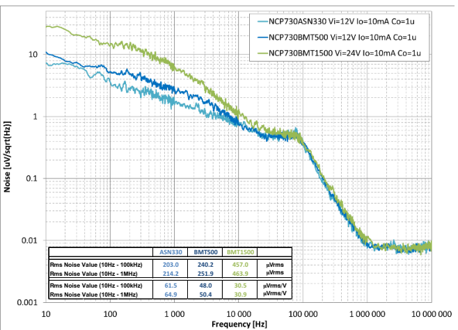
Figure 52. Noise – FIX, I_{OUT} = 10\text{ mA} , C_{OUT} = 1\text{ }\mu\text{F} , Different V_{OUT}
