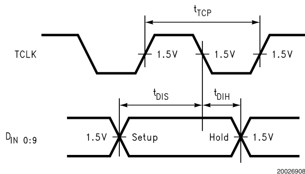
FIGURE 4. Serializer Setup/Hold Times
