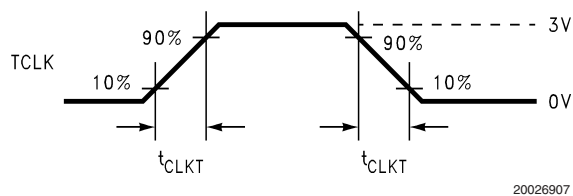
FIGURE 3. Serializer Input Clock Transition Time
