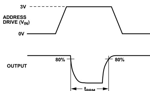
Figure 31. Break-Before-Make Delay, t_{\text{BBM}}
