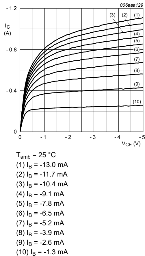
Fig. 11. BC807W-25: Collector current as a function of collector-emitter voltage; typical values
