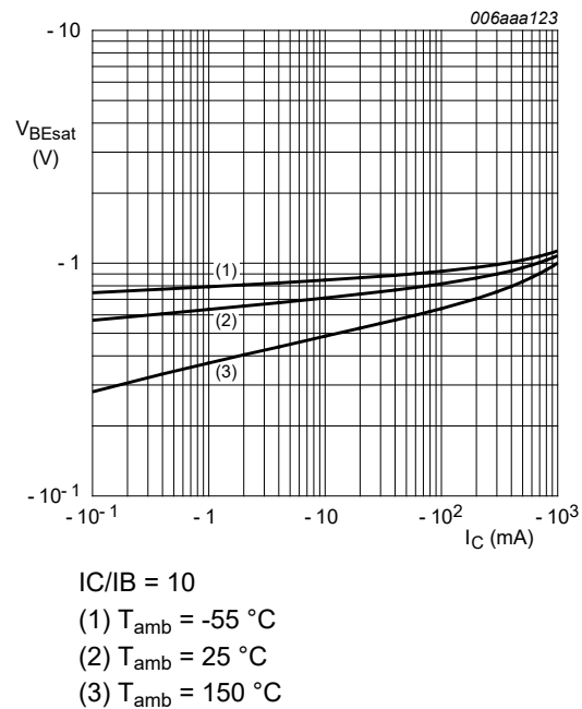
Fig. 9. BC807-25W: Base-emitter saturation voltage as a function of collector current; typical values
