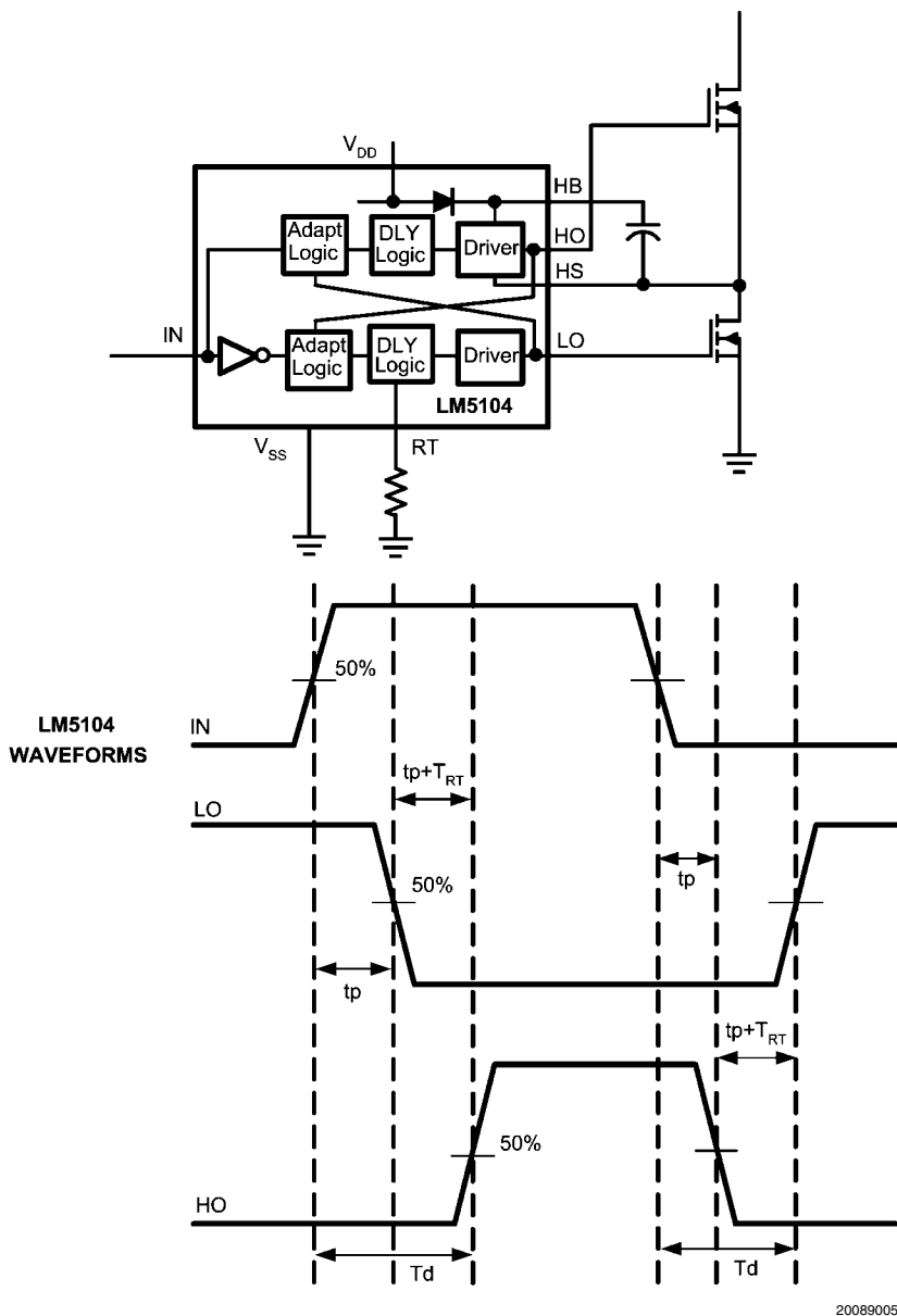
FIGURE 3. Application Timing Waveforms
