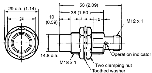
Fig.17: E2E-X10ME□-M1/F□-M1-N
