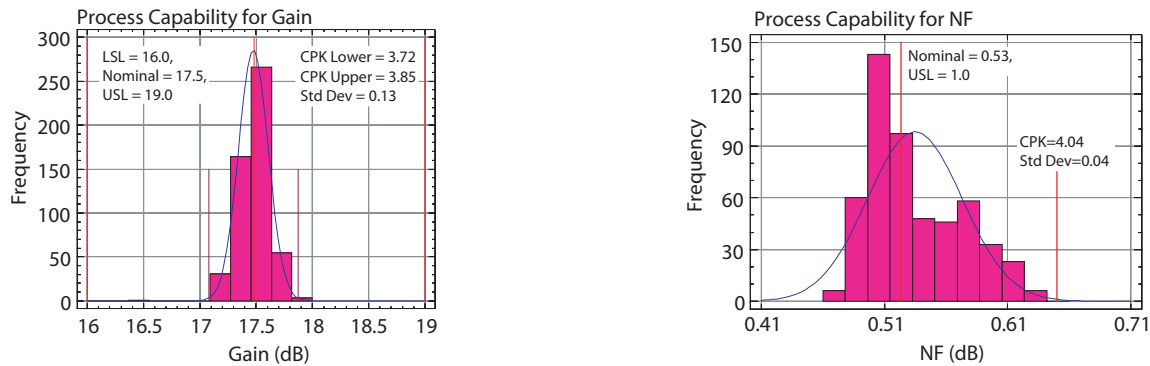
Figure 1. Gain distribution at 54mA
