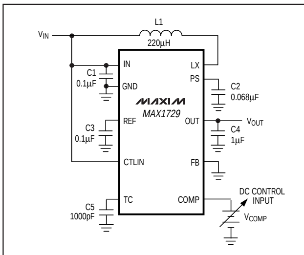
Figure 4. Using a DC Control Signal
