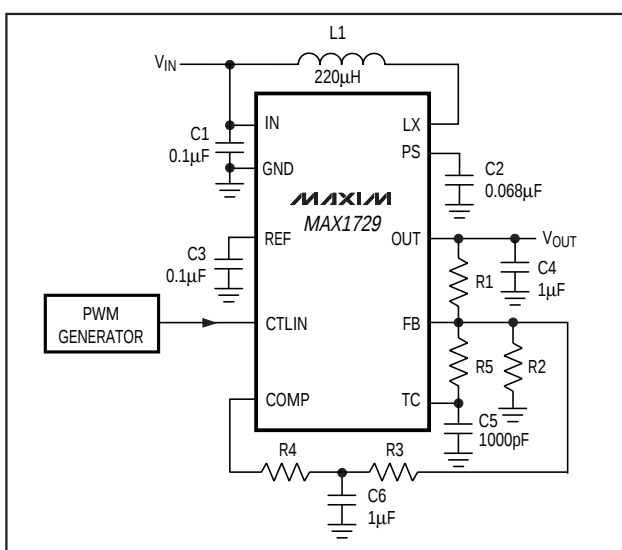
Figure 3. External Feedback Mode
