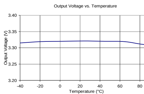
Figure 56: Output Voltage vs. Temperature
