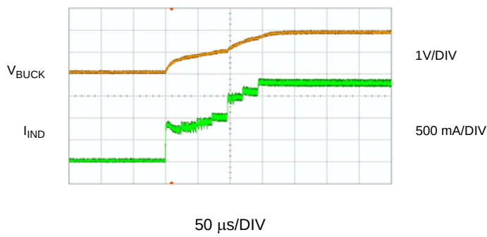
Figure 6: Inductor Current Steps at Startup
