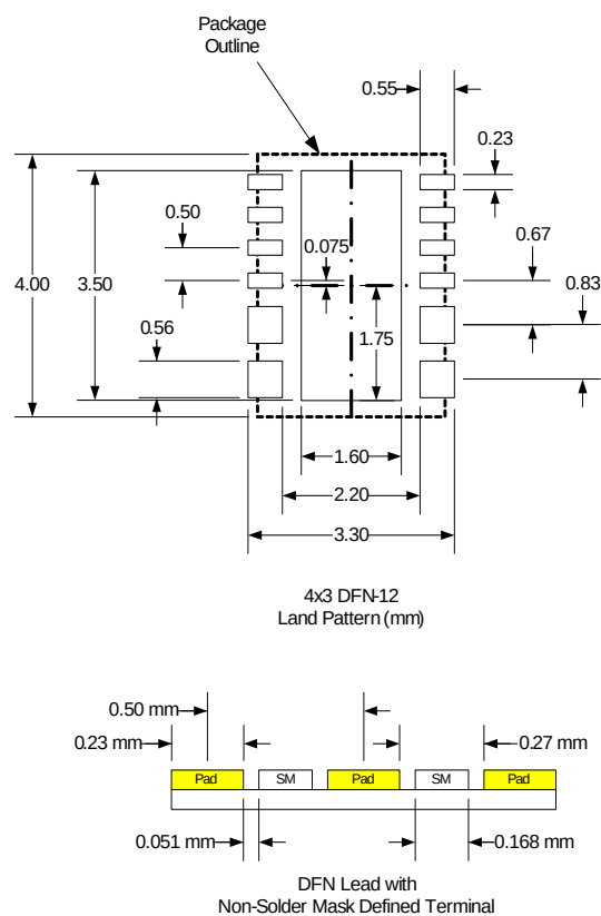
Figure 69: Recommended Solder Pad Layout
