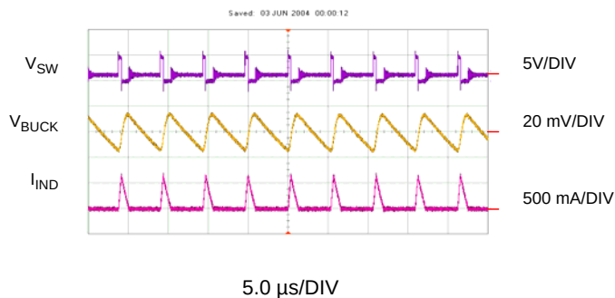
Figure 24: Switching Waveforms—DCM Mode
