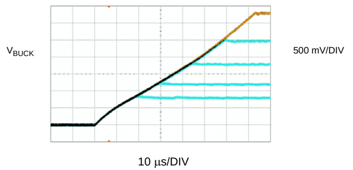
Figure 7: Soft Startup (0.8V, 1.2V, 1.8V, 2.5V, 3.3V)
