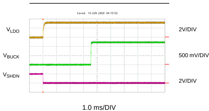
Figure 14: Startup Using the Shutdown Pin
