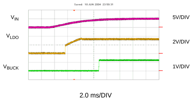
Figure 18: Input Voltage Soft Start
