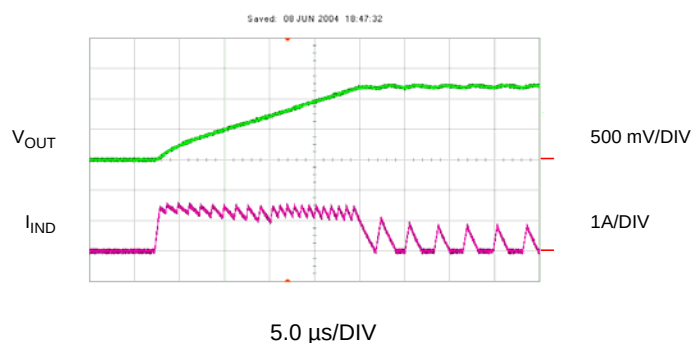
Figure 20: Step-Down Output Rise Time
