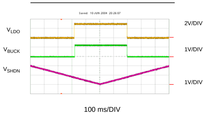
Figure 16: Enable Threshold at V_{IN} = 3.5\text{V}
