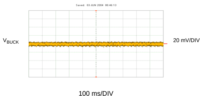
Figure 25: PWM Output Ripple Voltage
