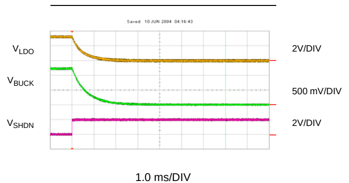
Figure 15: Turn Off Using the Shutdown Pin
