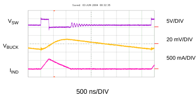
Figure 26: Switching Waveforms—DCM Mode-Zoom
