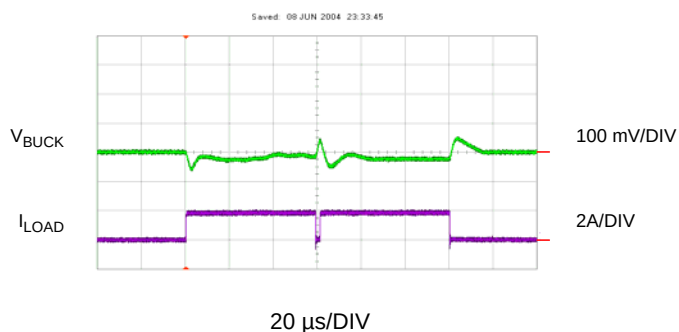
Figure 32: Double-Pulsed Load Response
