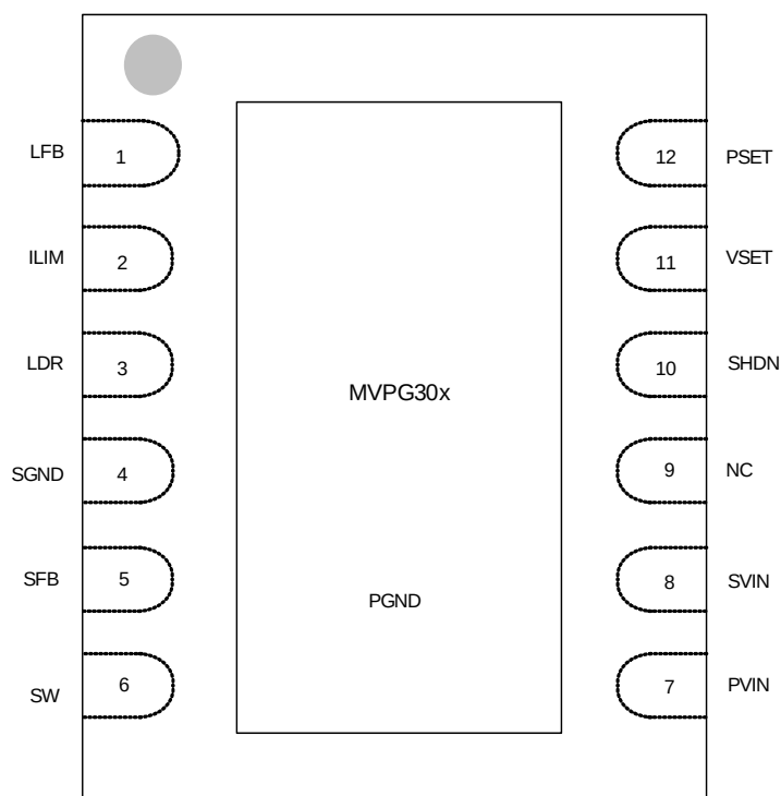
Figure 2: 12-Pin DFN Pin Diagram—MVPG30x Top View
