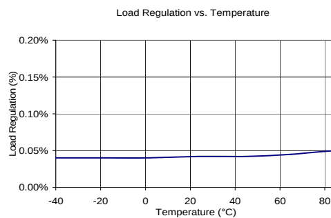
Figure 57: Load Regulation vs. Temperature
