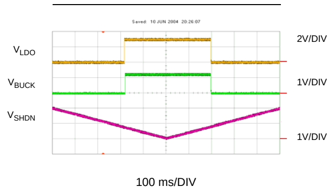
Figure 17: Enable Threshold at V_{IN} = 5.0\text{V}
