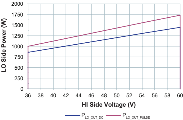
Figure 2 — Specified electrical operating area using rated R_{LO\_HOT}
