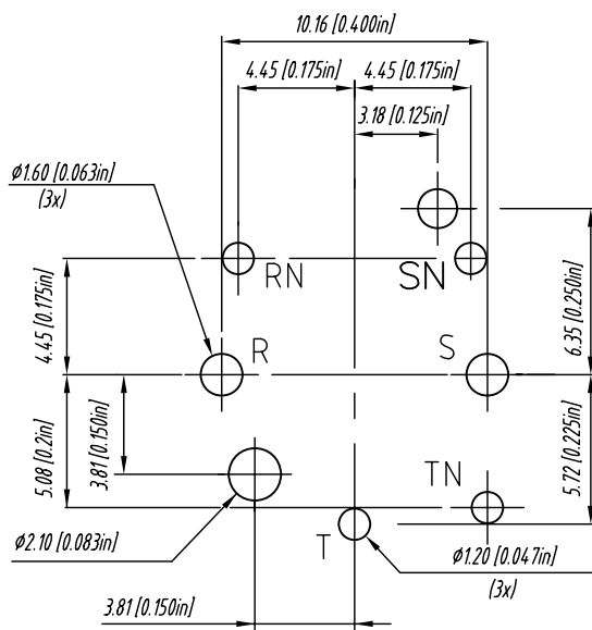
PCB-LAYOUT COMPONENT SIDE TOLERANCE: ±0.05mm [0.002"]
